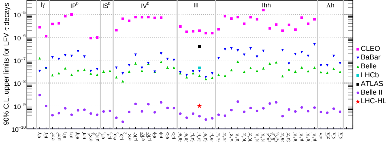
Figure 4: Current experimental limits on neutrinoless LFV \tau decays [86]. Also shown are the future projections at Belle-II [87] and at the HL-LHC [88].
